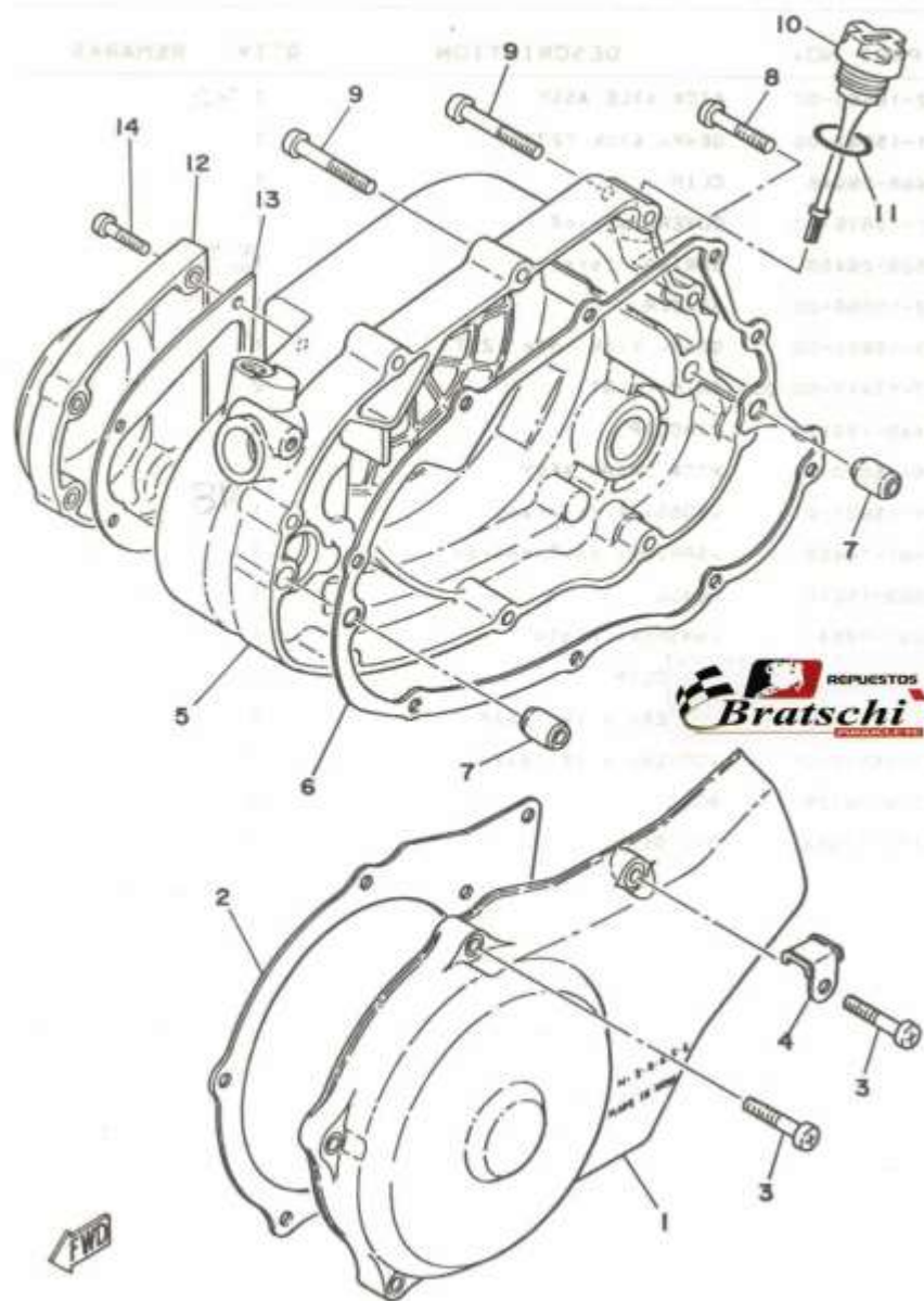
FIG. 9 CRANKCASE COVER
