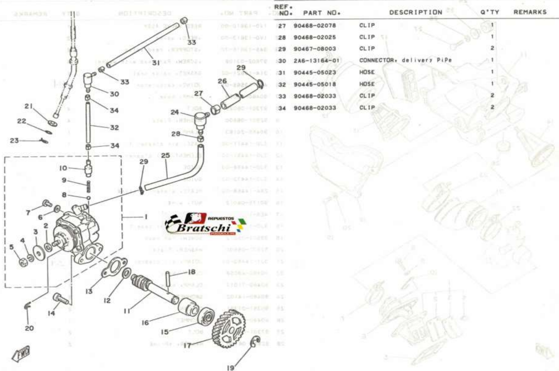
FIG. 4 OIL PUMP
