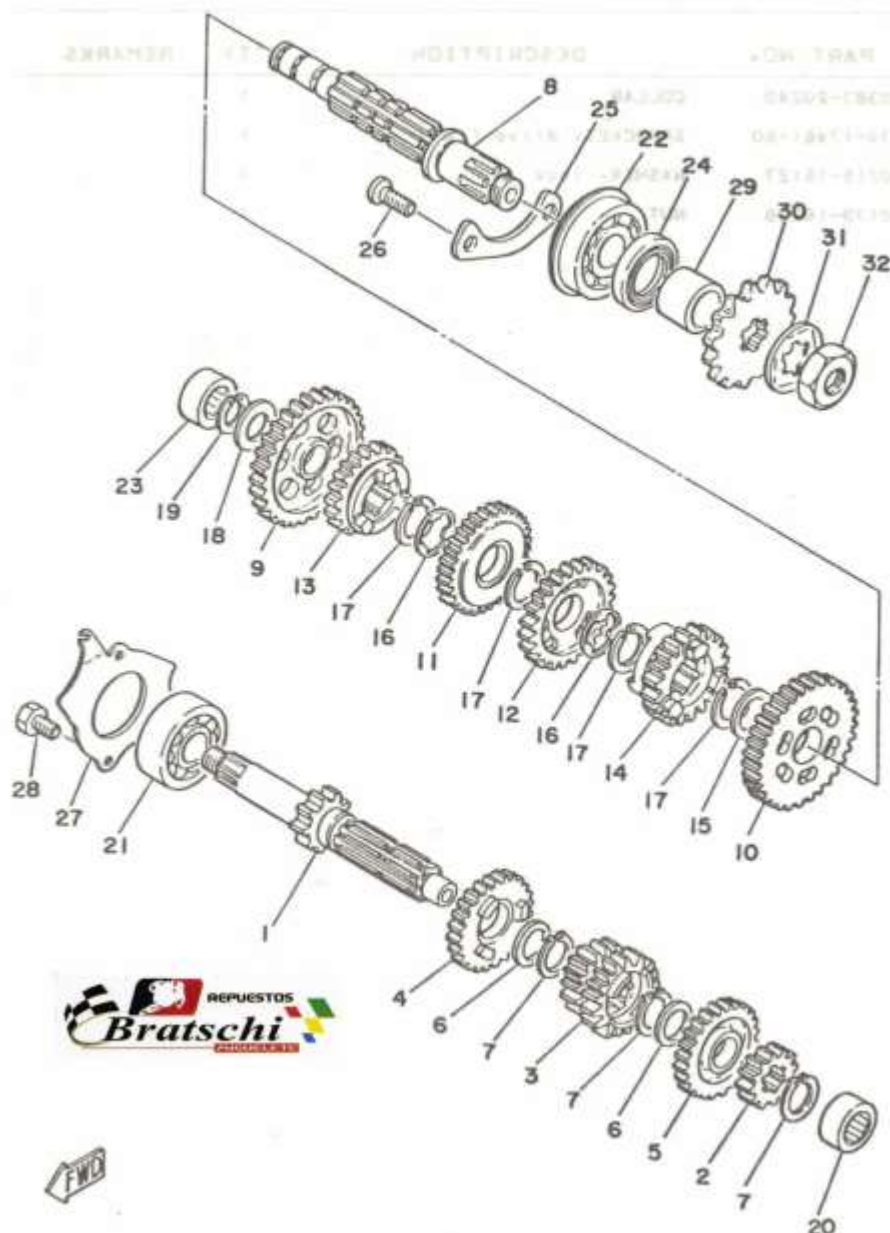
FIG. 12 TRANSMISSION
