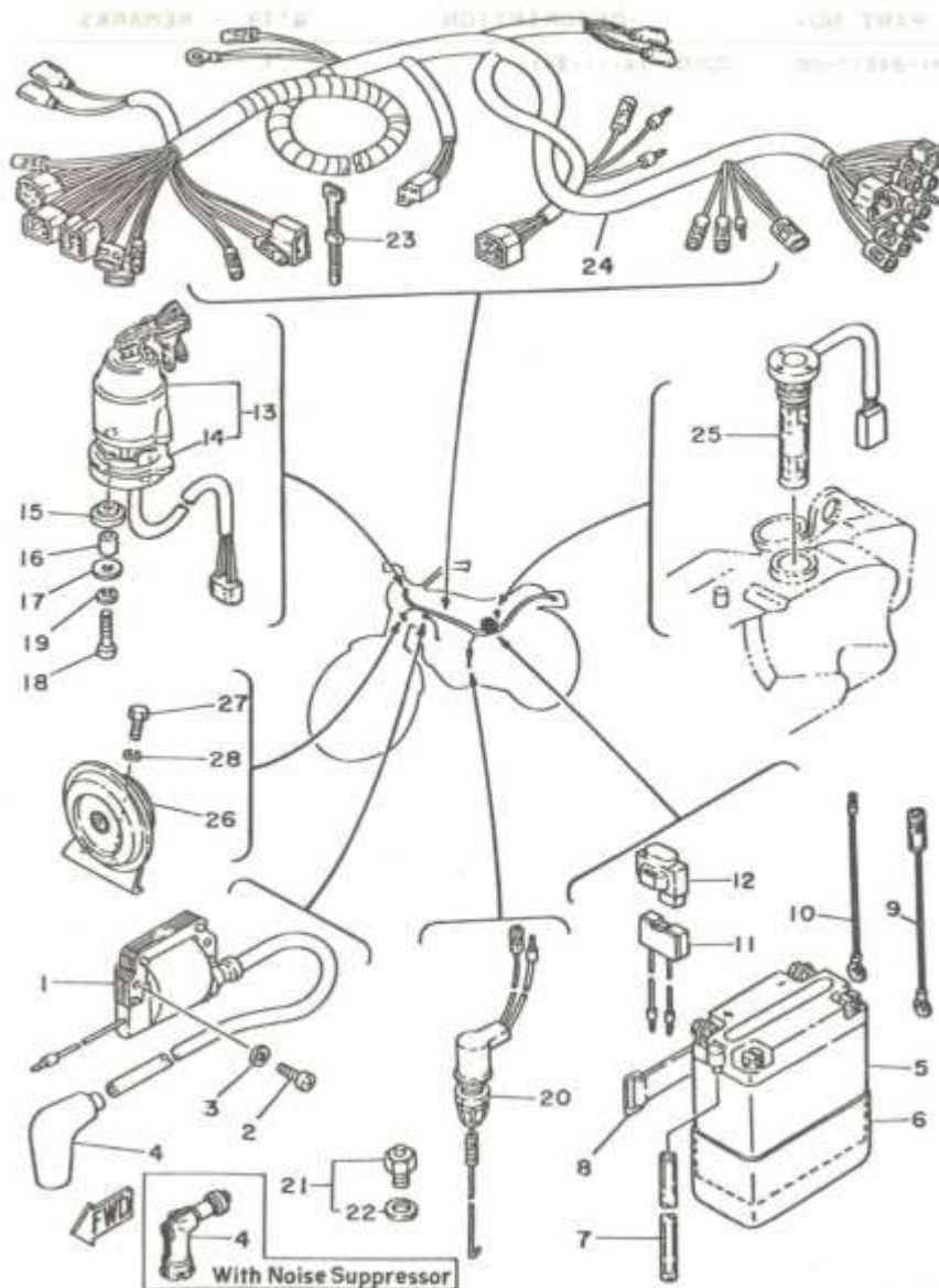
FIG. 34 ELECTRICAL 1
