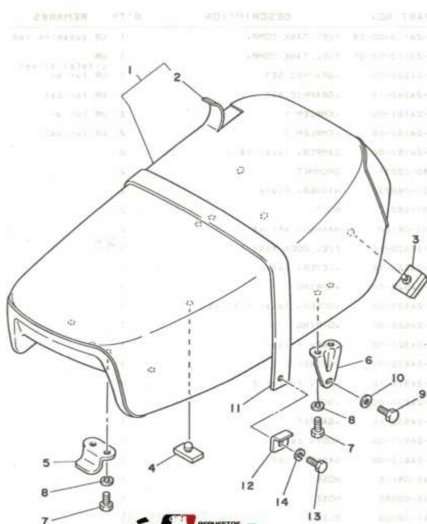
FIG. 25 SEAT
