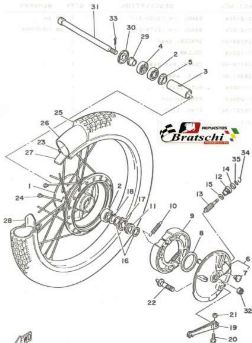
FIG. 26 FRONT WHEEL
