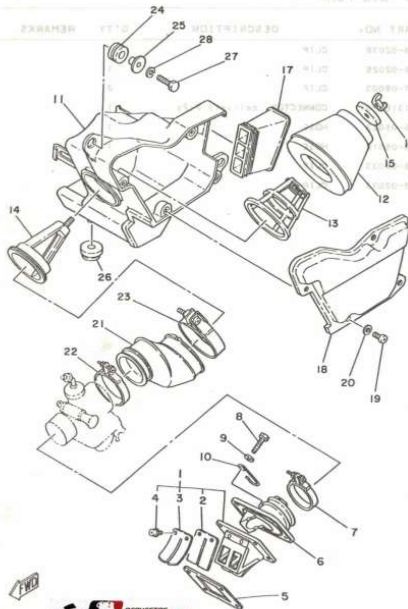
FIG. 5 INTAKE
