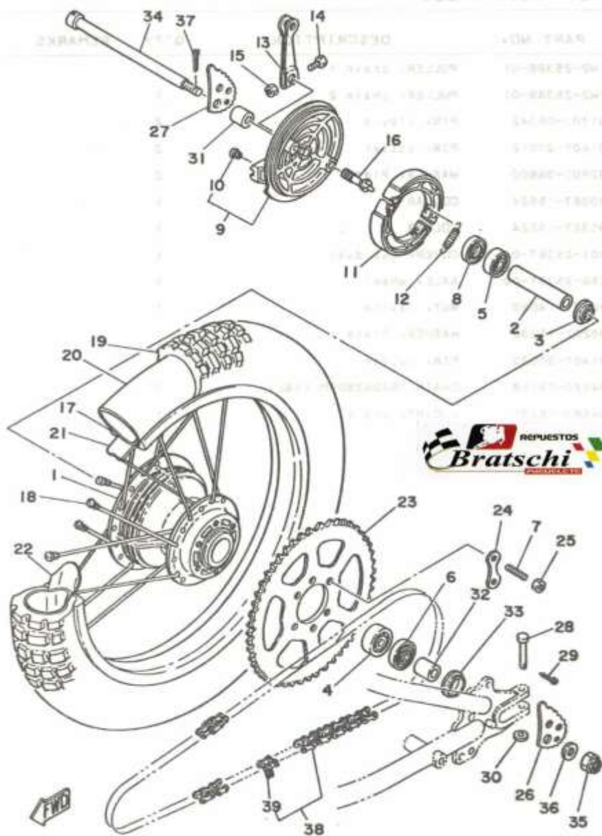
FIG. 27 REAR WHEEL
