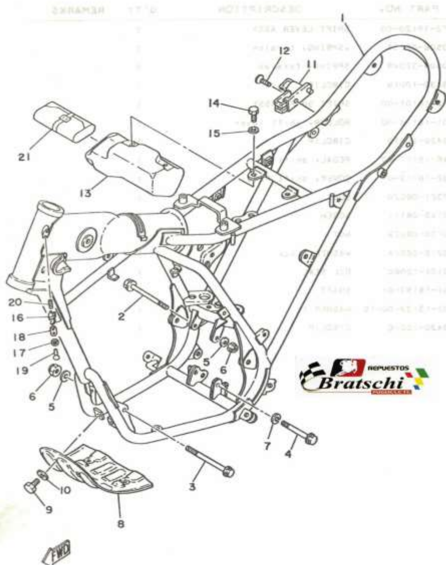
FIG. 16 FRAME. TOOL
