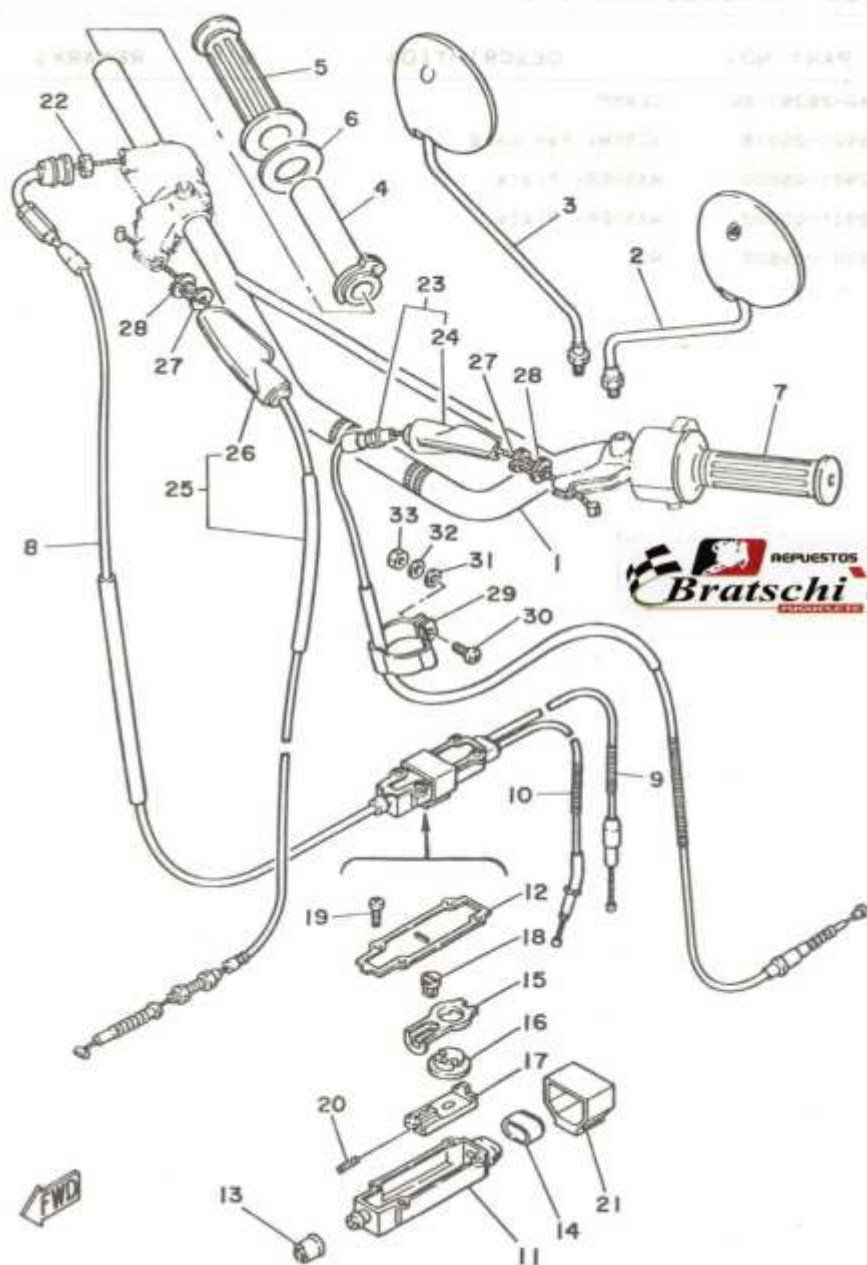
FIG. 28 HANDLEBAR.CABLE
