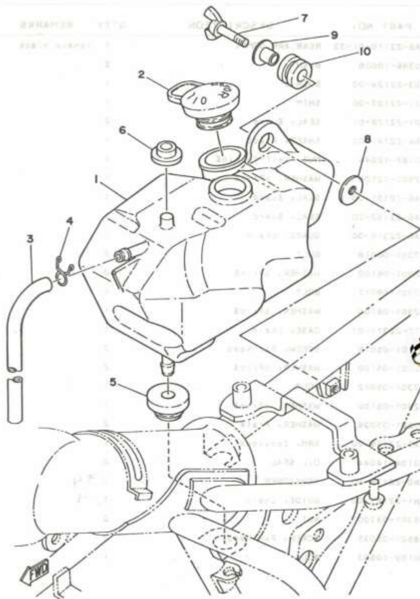
FIG. 19 OIL TANK
