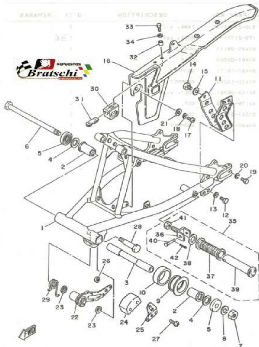
FIG. 20 REAR ARM
