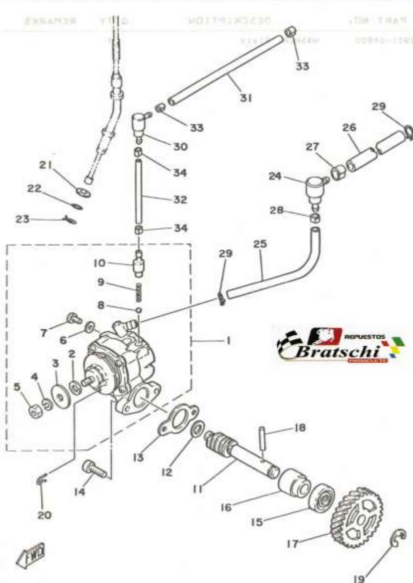
FIG. 4 OIL PUMP
