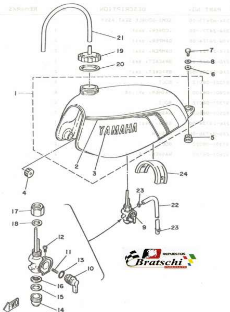
FIG. 24 FUEL TANK
