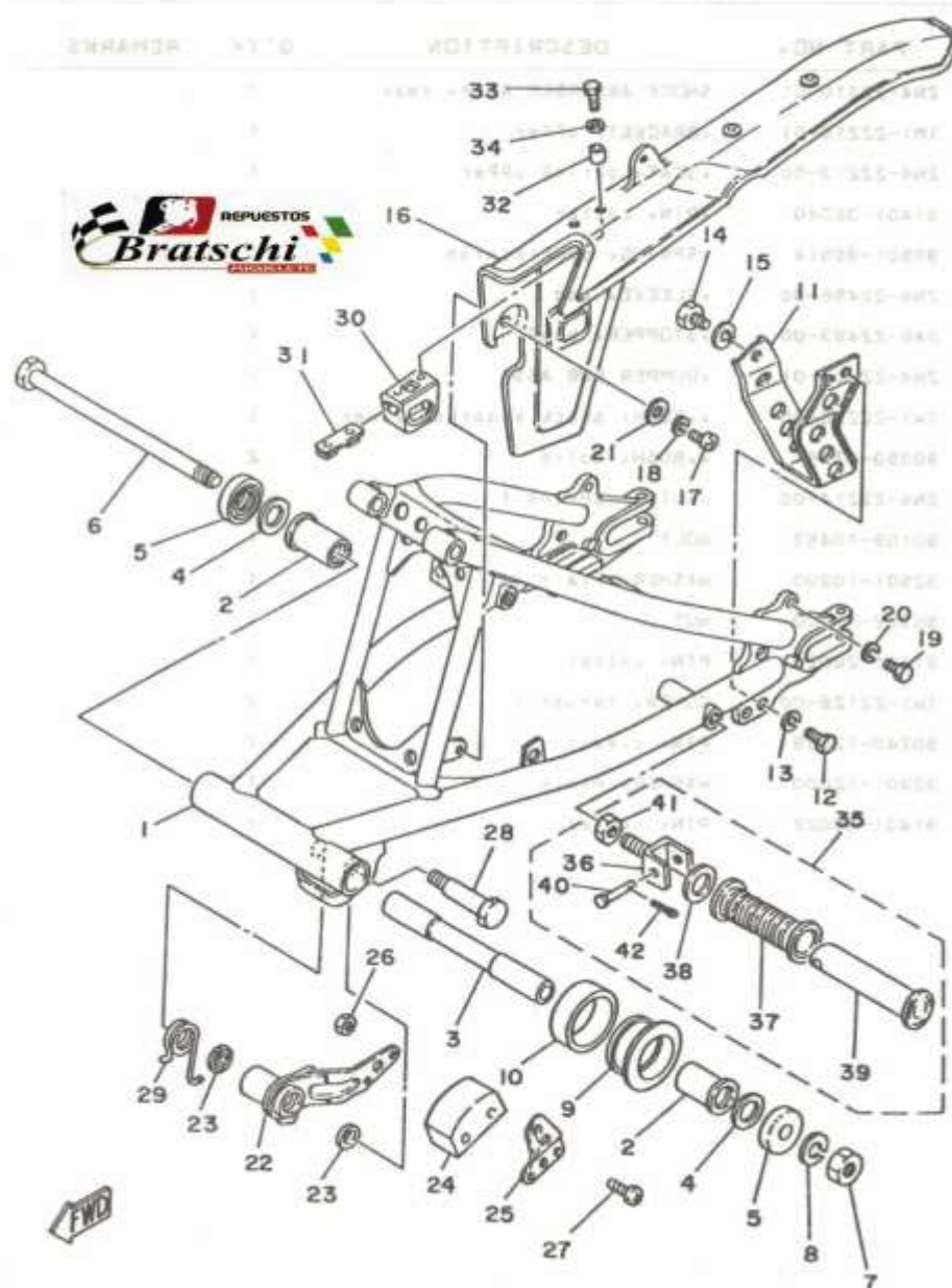
FIG. 20 REAR ARM
