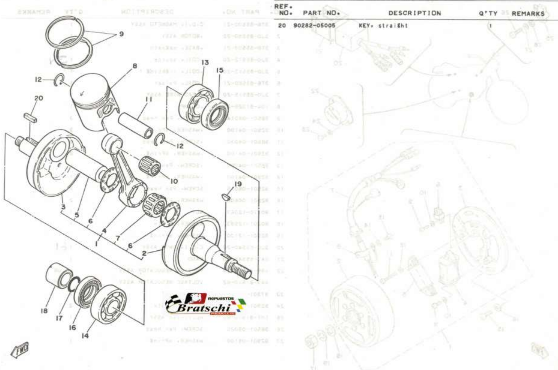
FIG. 2 CRANKSHAFT-PISTON
