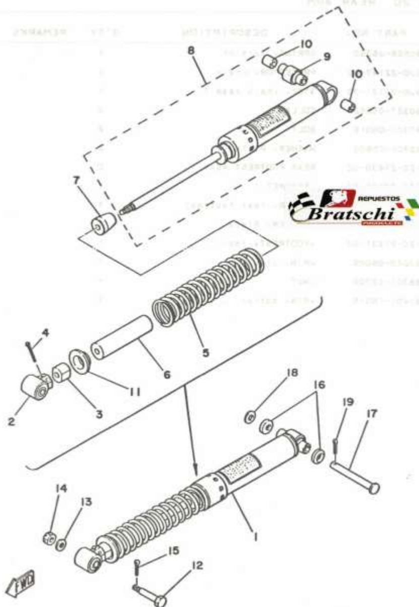
FIG. 21 REAR SUSPENSION
