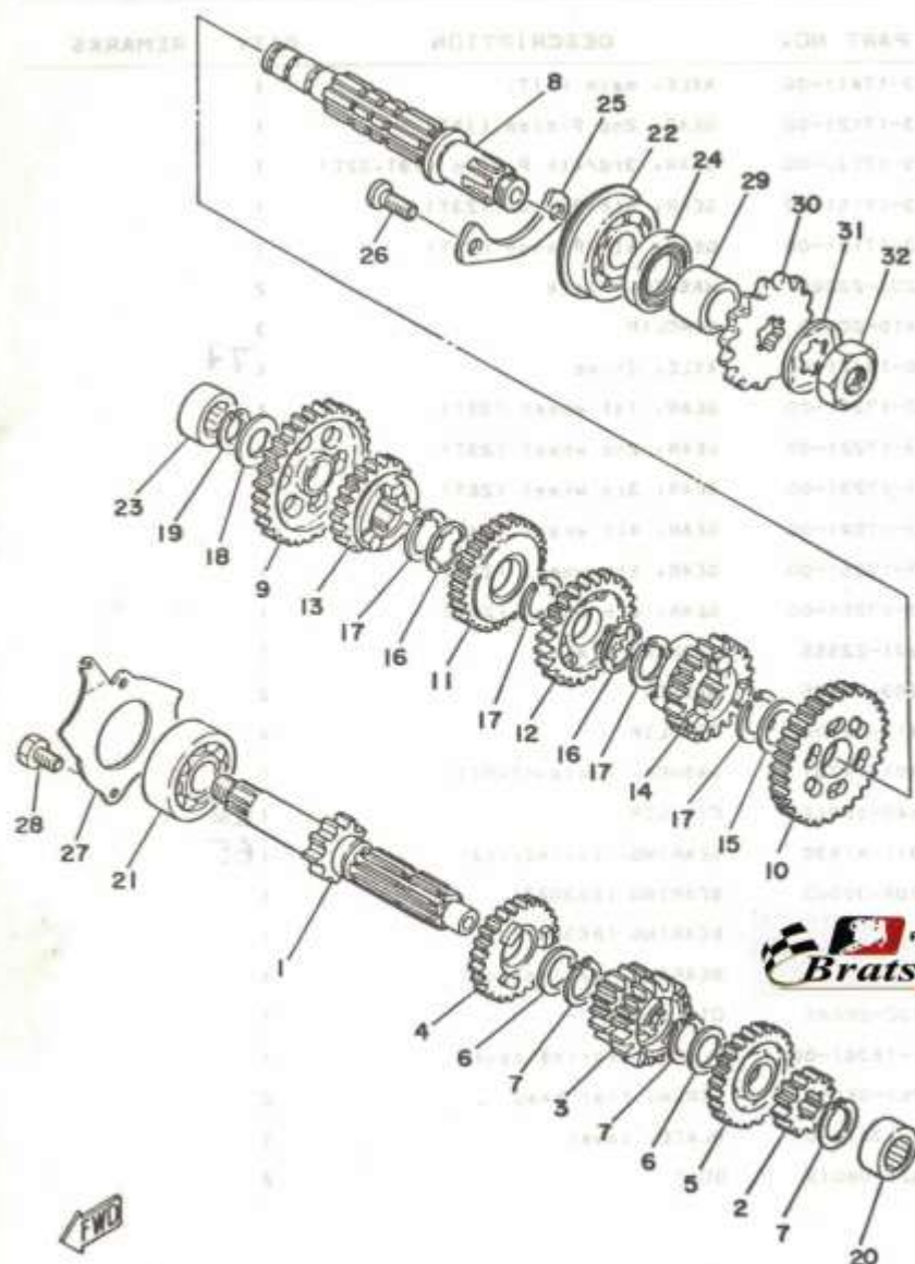
FIG. 12 TRANSMISSION
