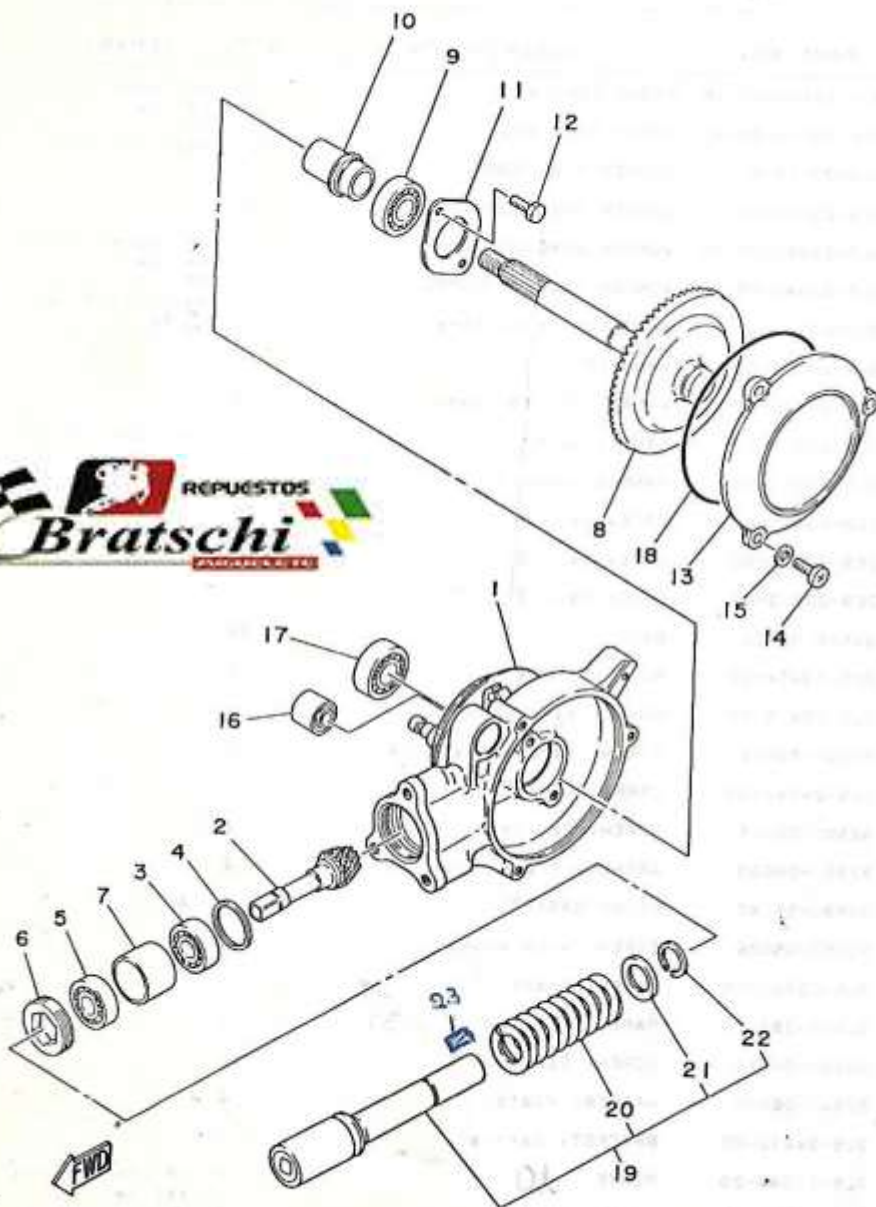
REF. NO. PART NO. DESCRIPTION Q'TY REMARKS 1 3L5-46151-00 HOUSING, drive shaft 1 2 3L5-46121-00 GEAR, drive Pinion 11 1 3 93306-20111 BEARING 29 1 4 3L5-46127-00 SHIM, drive Piston 12 1 5 93306-20109 BEARING (B6201) 1 UR 93306-20110 BEARING (B6201) 1 UR 6 90149-35133 SCREW 12 1 7 90560-25185 SPACER 1 8 3L5-46110-00 RING GEAR COMP. (57T) 31 1 9 93306-20205 BEARING (B6202) 1 UR 93306-20209 BEARING (B6202) 1 UR 10 3L5-25317-00 SPACER, bearing 1 11 3L5-46114-00 PLATE, cover 1 12 97311-06016 BOLT 2 13 3L5-46154-01 COVER, housing 1 14 92501-06015 SCREW, Pan head 3 15 92901-06600 WASHER, Plate 3 16 164-22216-00 102-22423-00 BUSH, rear shock absorber 1 17 93306-20203 BEARING (B6202RS) 1 18 93211-05393 O-RING 1 19 3L5-46171-00 SHAFT DRIVE ASSY 1 20 90501-60556 SPRING, compression 1 21 3L5-18473-00 RETAINER, spring 12 1 22 93440-17073 CIRCLIP 1 23 93540-16132 Pinon 40 4 www.bratschirepuestos.com
